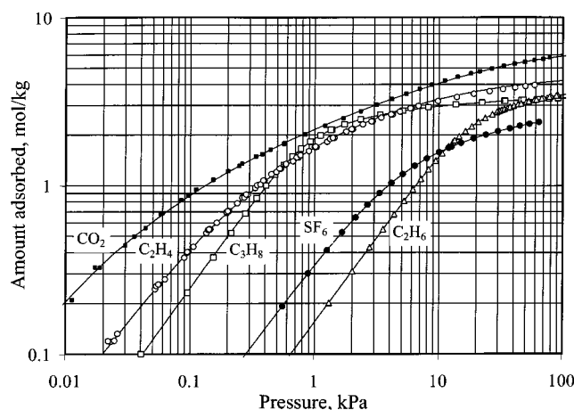
Figure 1. Experimental adsorption isotherms on NaX.
