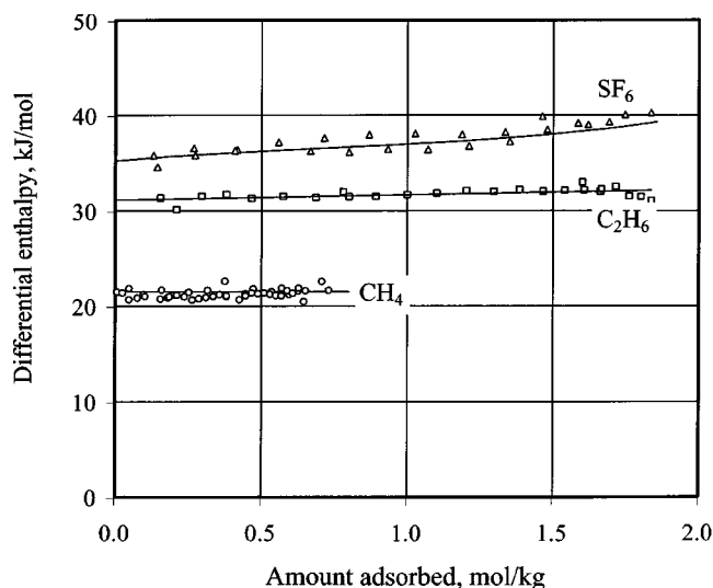
Figure 4. Experimental differential enthalpies (isosteric heats) on silicalite at 298 K.
