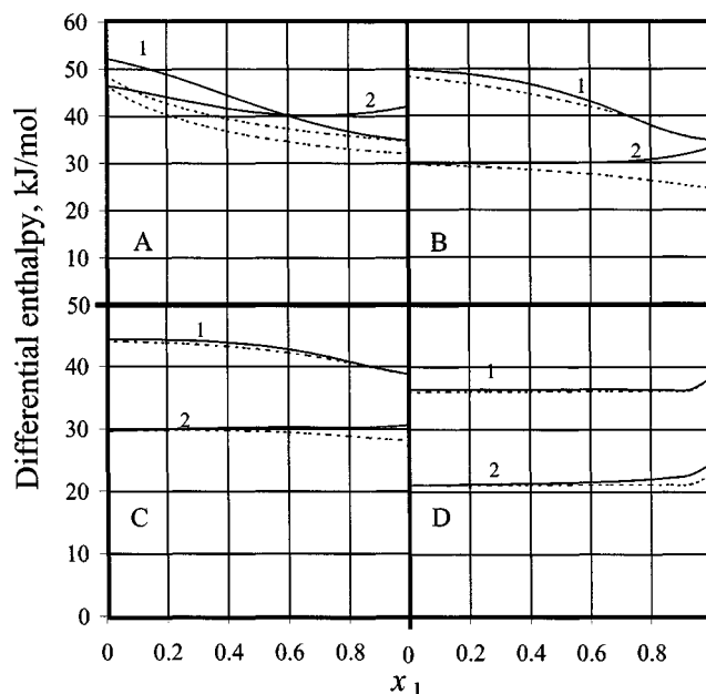
Figure 13. Isothermal (295 K), isobaric (13.3 kPa) differential enthalpies (isosteric heats).
