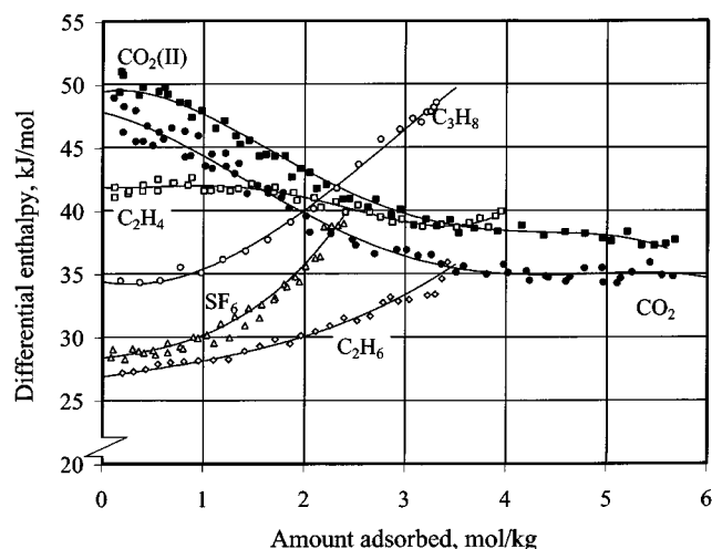
Figure 3. Experimental differential enthalpies (isosteric heats) on NaX at 298 K.
