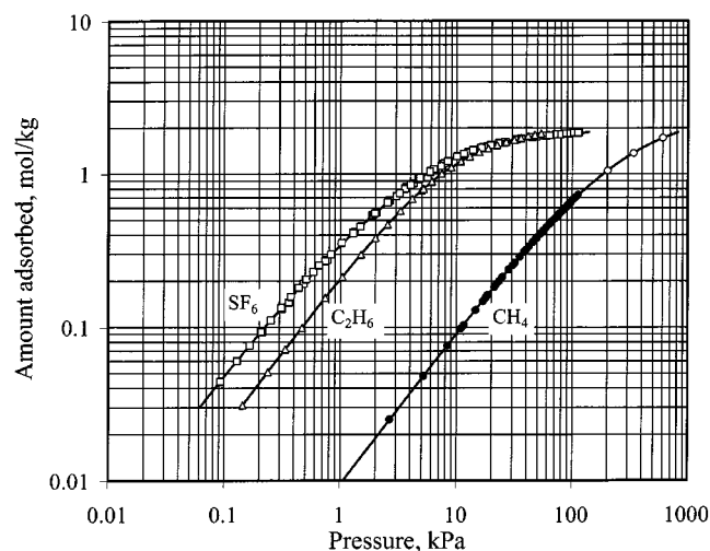
Figure 2. Experimental adsorption isotherms on silicalite.
